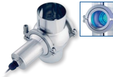
Inline housing with sight glass and LED illumination unit
